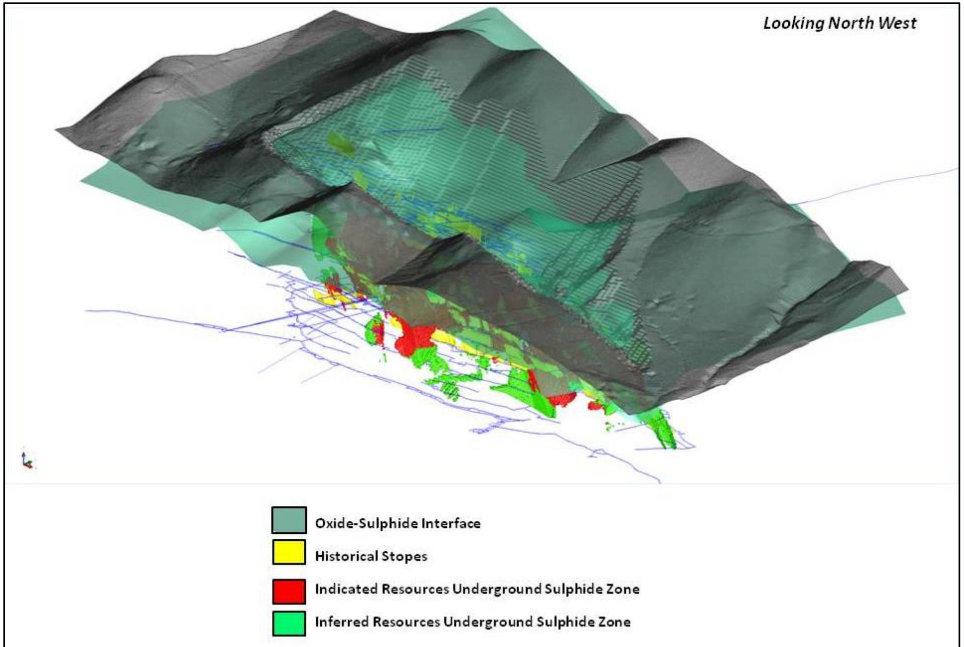
Figure 3: Optimized Open Pit Shell showing oxide sulphide interface historical underground workings and underground sulphide resources.
