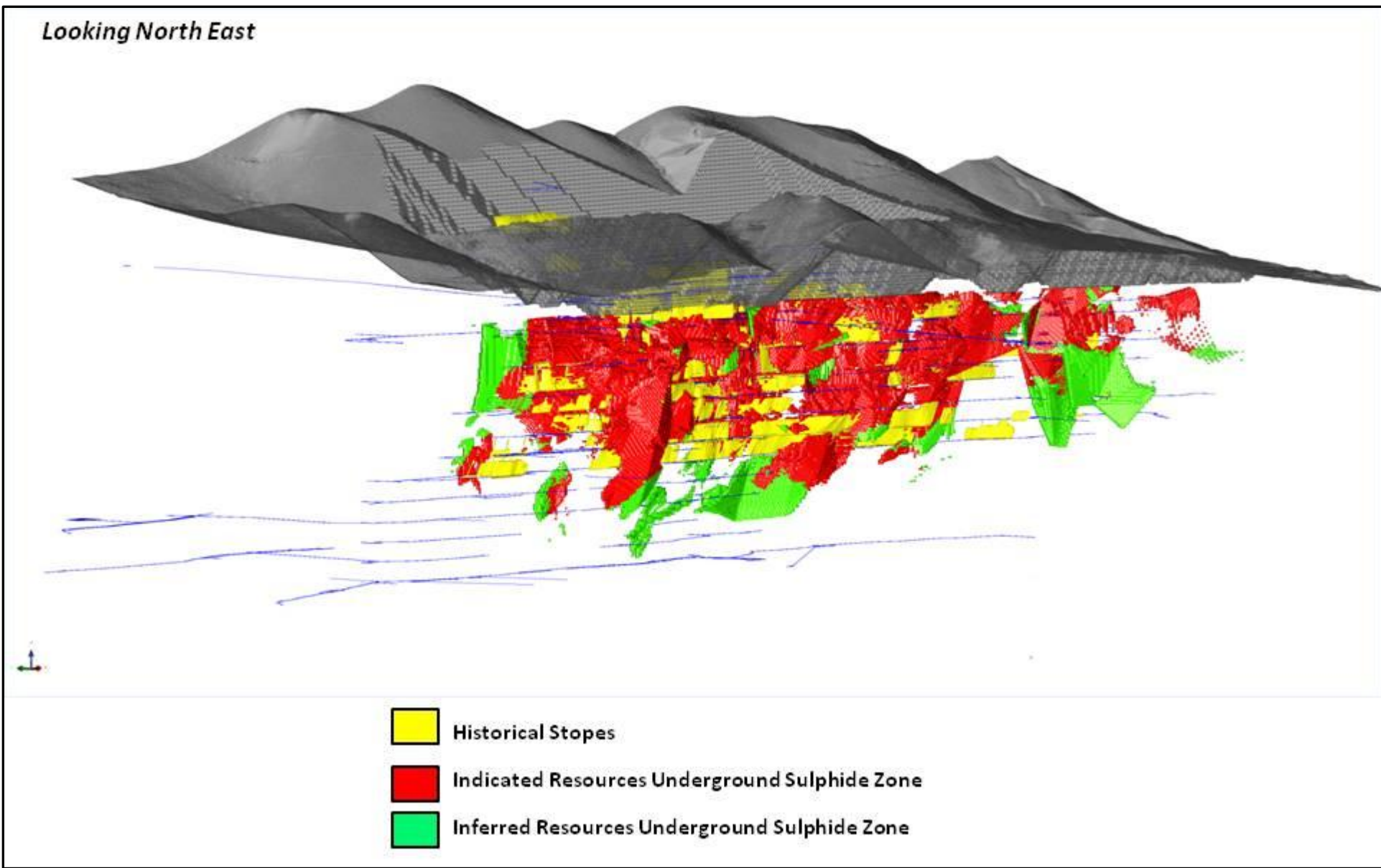
Figure 4 Underground sulphide resources showing historical stopes, level development and Open Pit Shell.
