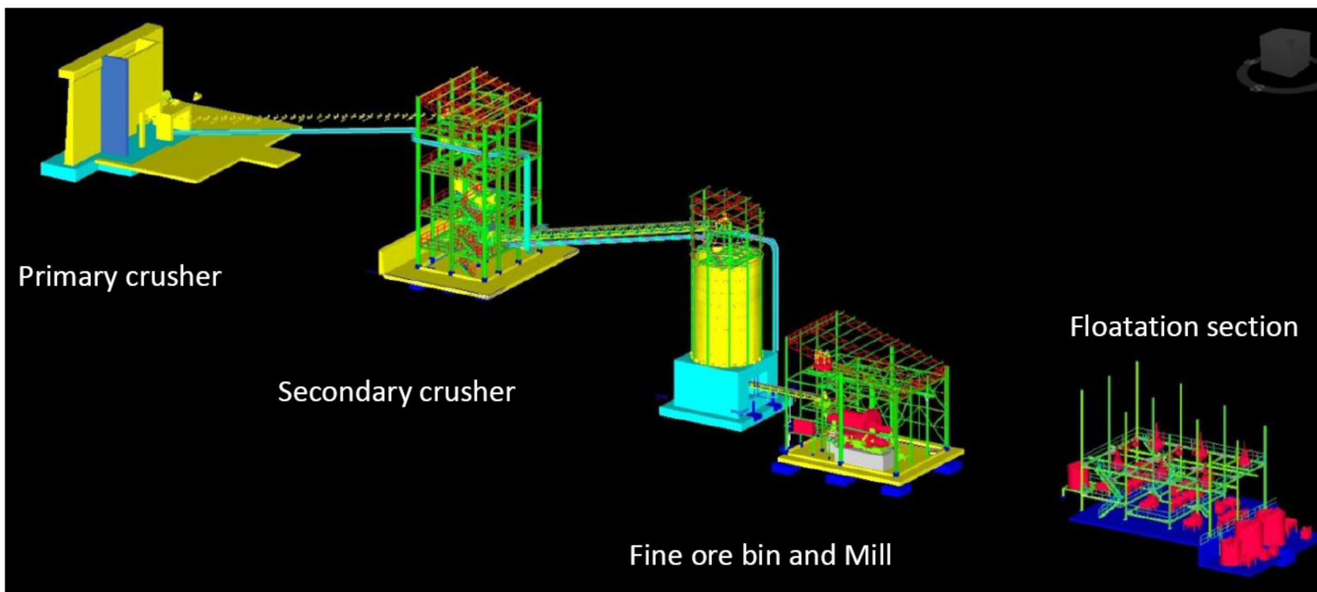
Figure 5. An isometric view of the main features of the pilot concentrator
