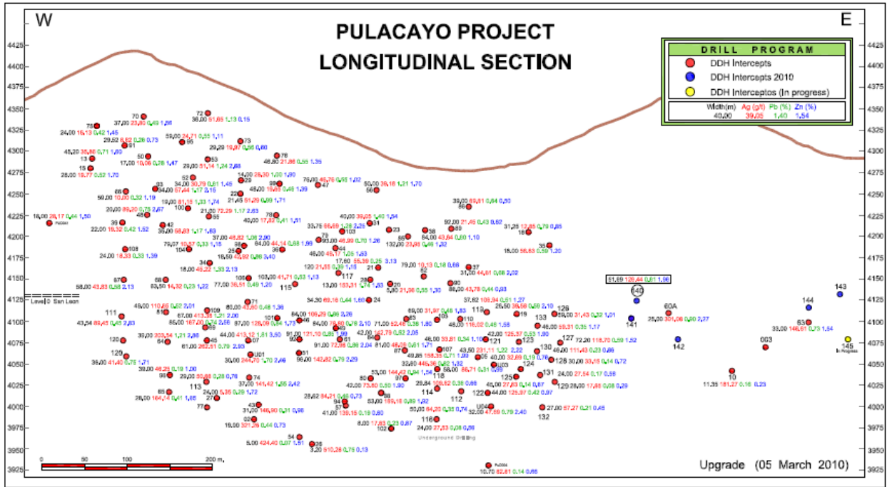
Figure 1 Vertical Longitudinal Section Pulacayo Deposit
