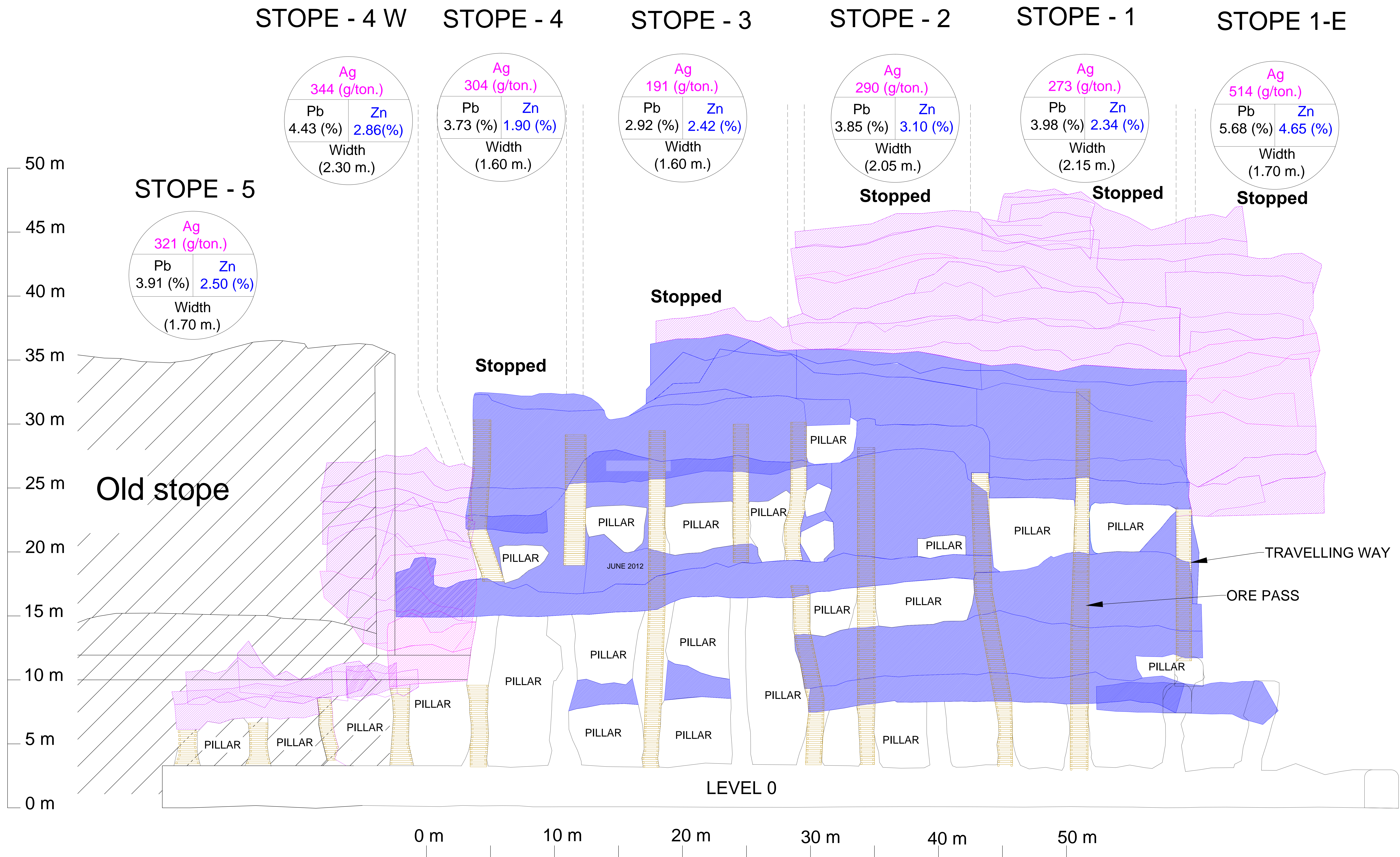
APOGEE SILVER PULACAYO PROJECT FIGURE 3: Long Section of Ore Body 6 Stopes Area
