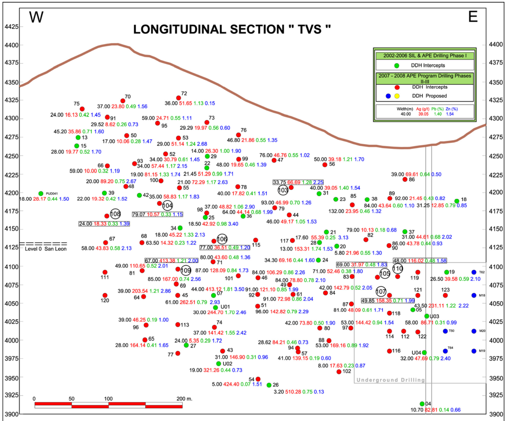
Figure 2: Vertical Longitudinal Section of the upper part of the Tajo Vein System, showing intersection locations and planned drill holes, including underground drilling.
