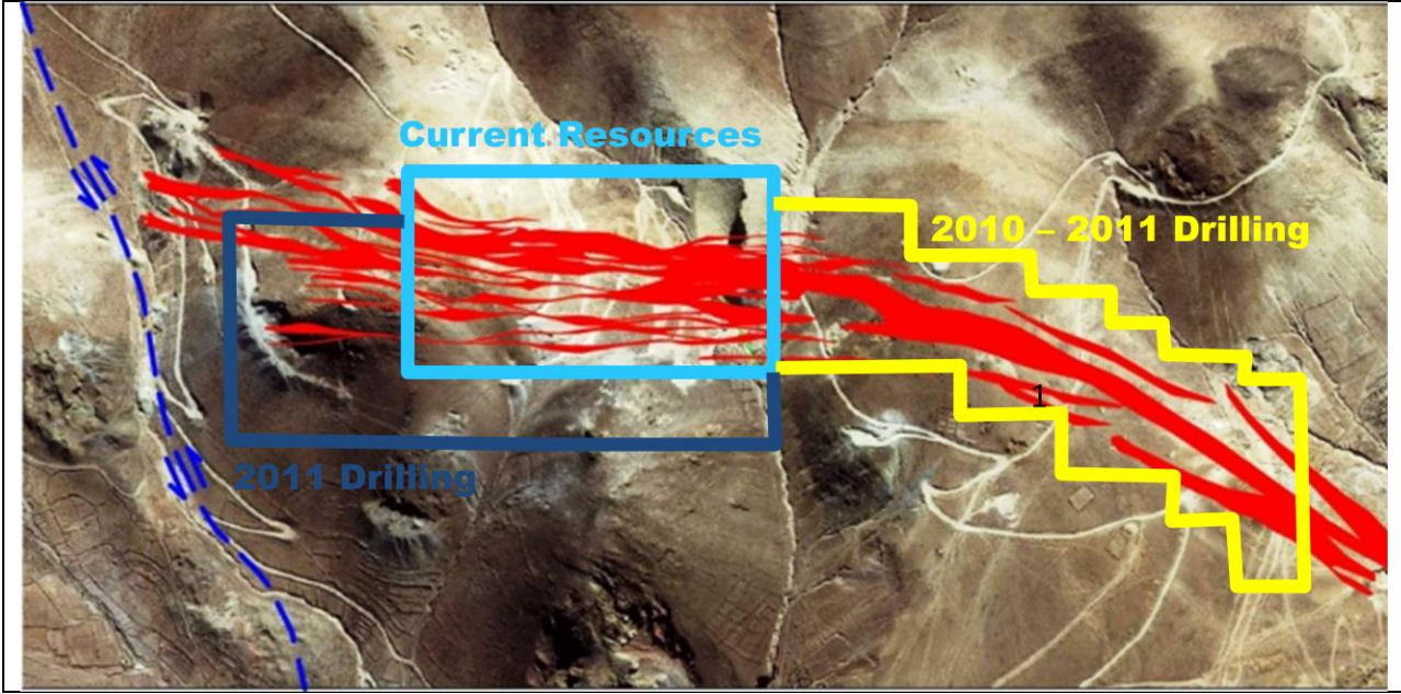
Figure 2: Tajo Vein System, Plan View.
