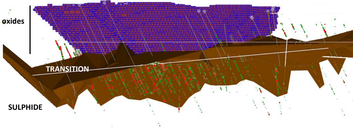
Skematic view of transition and oxide ore as it underlies the oxide open pit area
