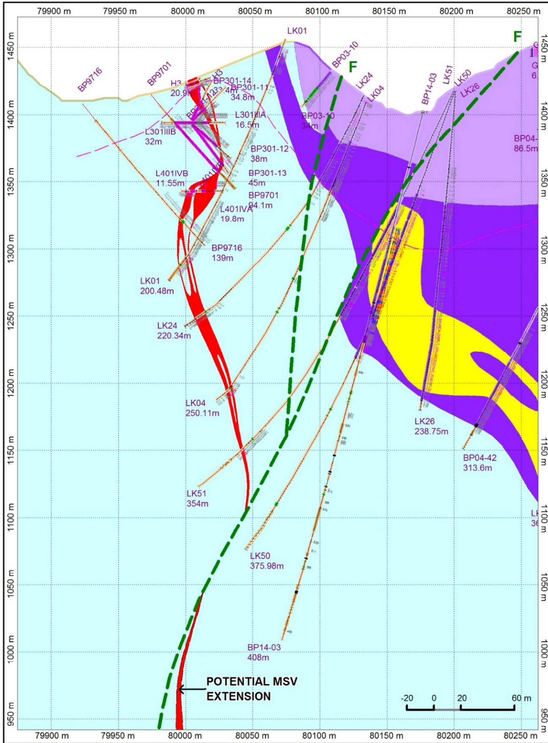
Figure 4. Ban Phuc Cross Section 49800mE showing offset in MSV and ultramafic rocks
