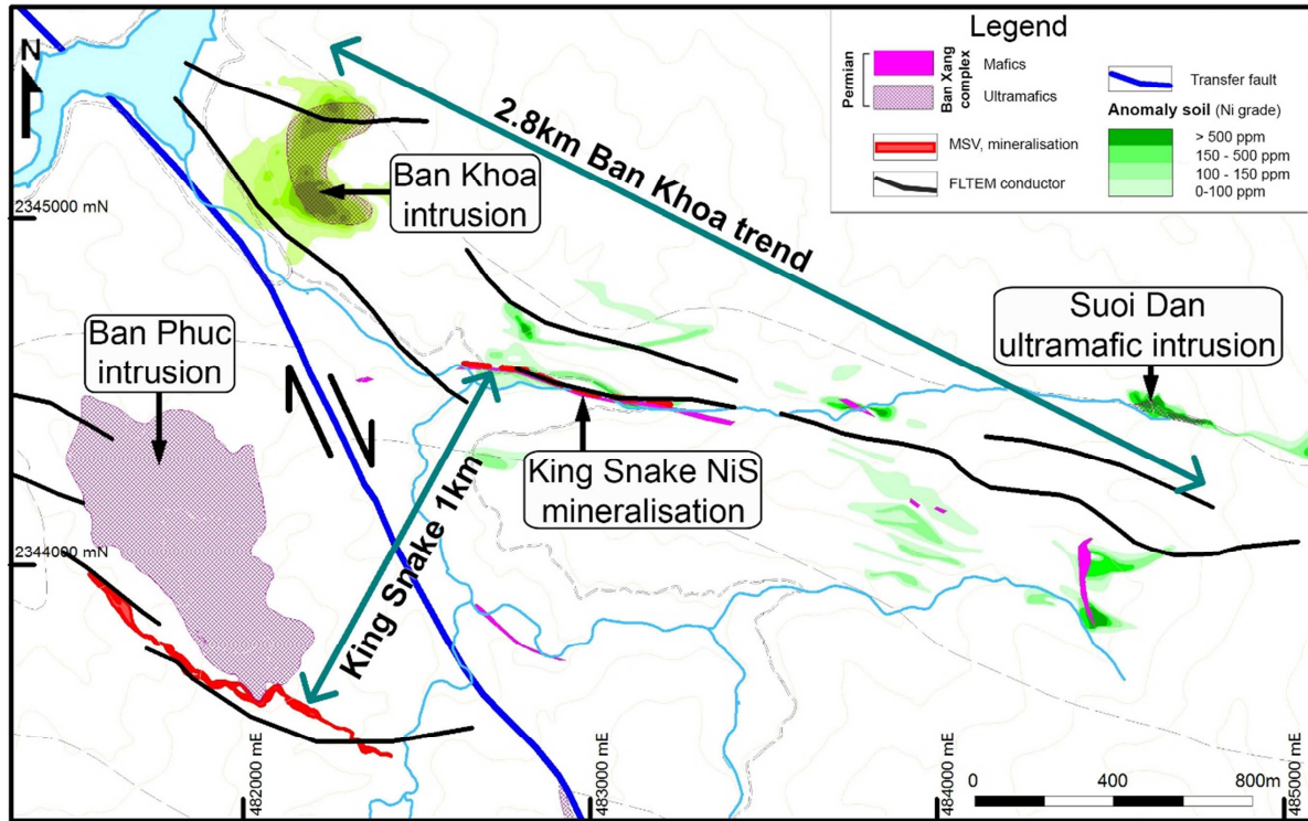
Figure 7. Ban Khoa trend prospect geology with geophysics (FLTEM) and surface geochemical anomalism.
