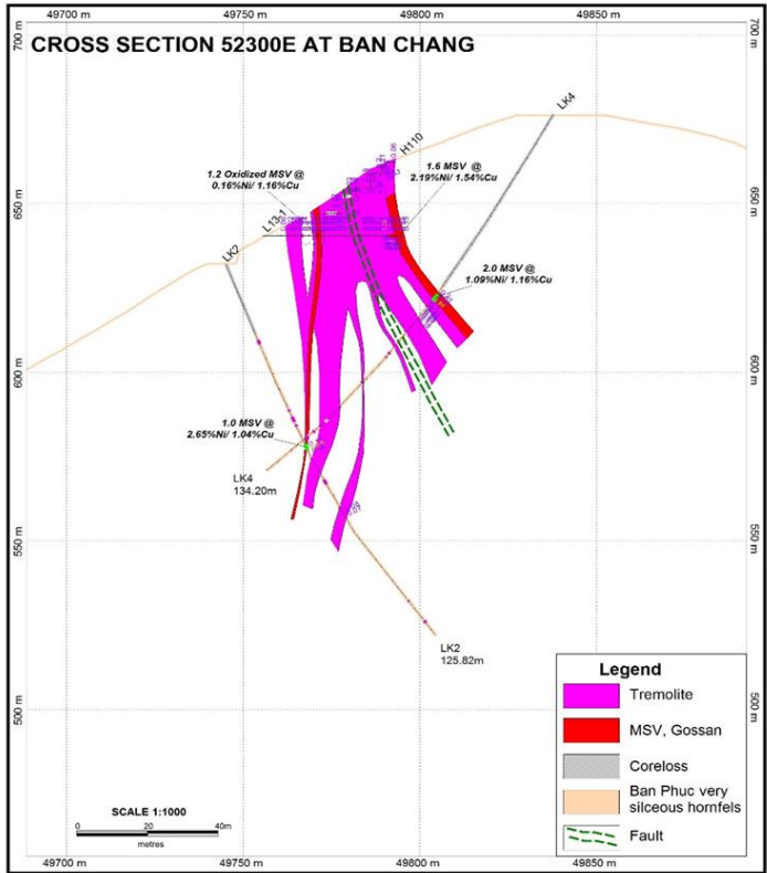
Figure 2: Updated cross section 50,330E based on the back mapping results of adit BCL13
