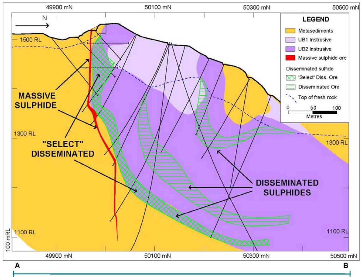
SECTION "A-B" (50000E) - LOOKING WEST
