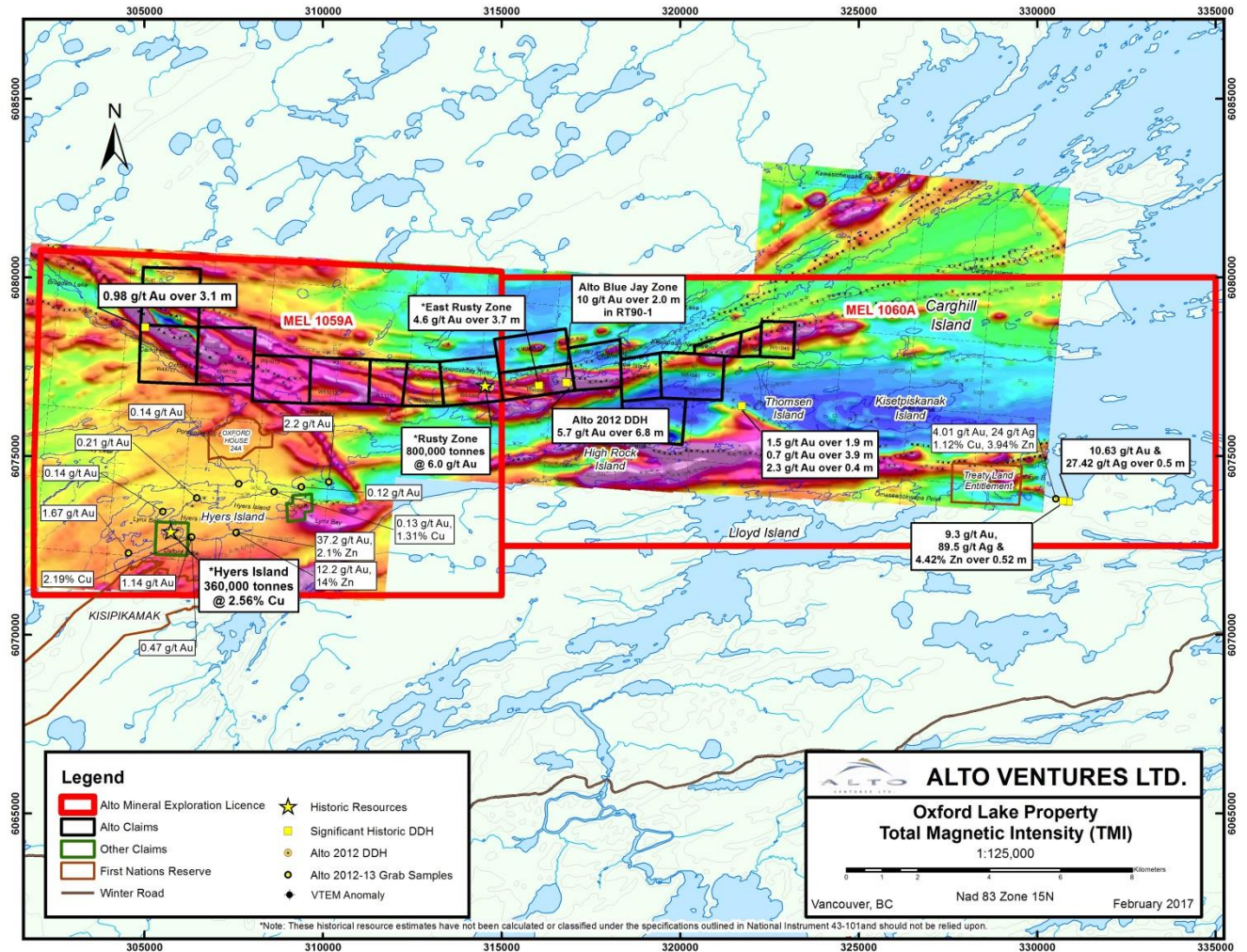
Figure 1 Oxford Lake property Total Magnetic Intensity map showing the extensive 30 km trend of magnetic highs, intensifying to the west of the Rusty Gold Deposit. Map also shows locations of numerous other gold occurrences and the Hyers Island and Cat Eye Bay volcanogenic massive sulphide targets.
