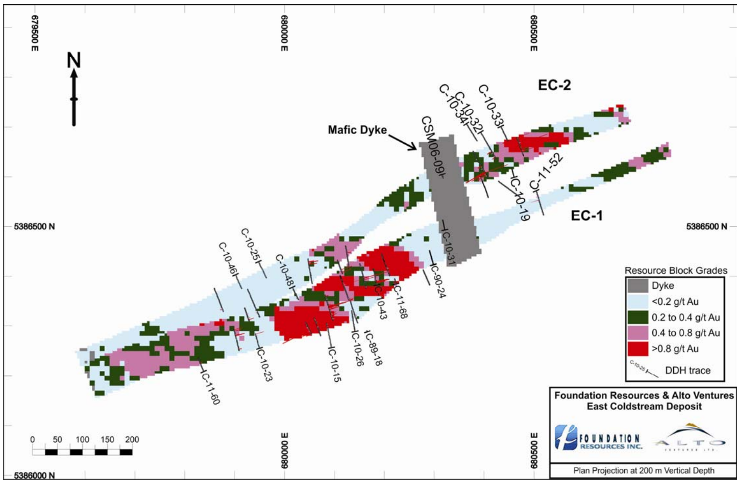
Figure 1. Plan View of the East Coldstream Gold Deposit showing the gold grade distribution of EC-1 and EC-2 at the 200 m vertical depth. Note the apparent convergence of the two mineralized horizons to the west.
