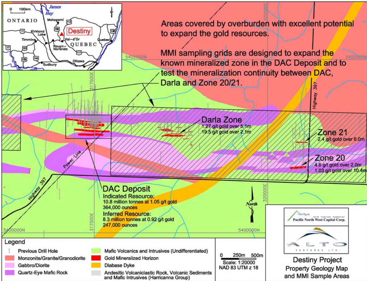
Figure 1 Property Geology Map and MMI Sample Areas
