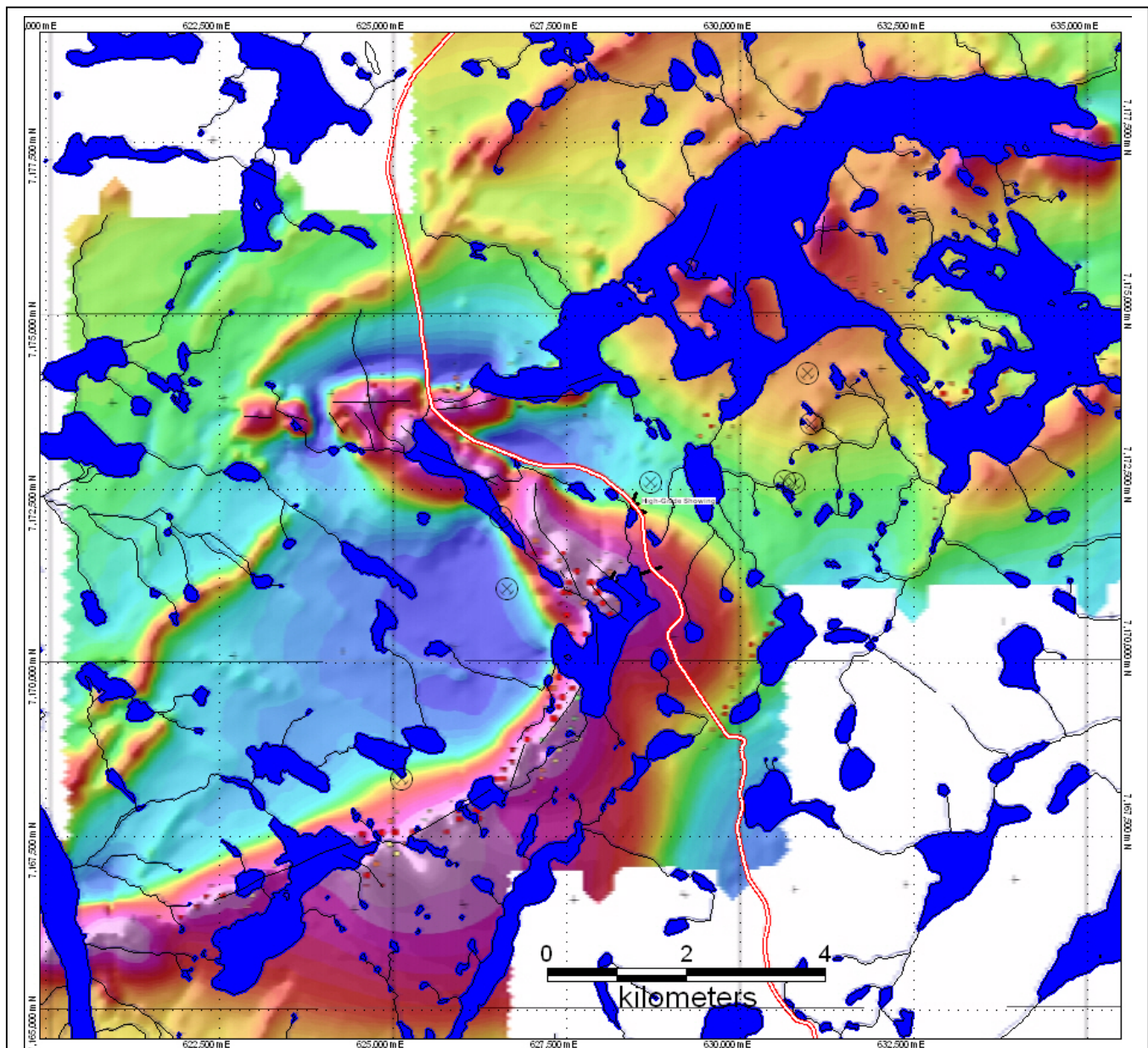
Figure 2: Revised analysis of the airborne geophysical responses in the Greyhound area. Red dots are strongest anomalies, caused by iron formation in some cases. Yellow and turquoise dots are more discreet anomalies, probably caused by sulfide bodies.
