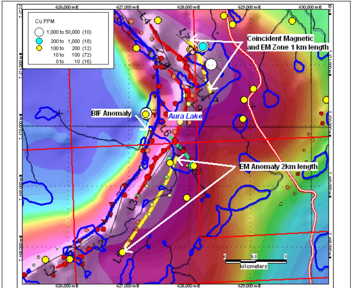
Figure 3: Details of geophysical data for the Aura Lake area; the blue line represents the BIF, which is adjacent to the Zn-Ag samples noted in Figure 1. The red and yellow lines are more typical of massive sulfide – type anomalies, and for example have coincident copper anomalies in surface samples (white, yellow and turquoise dots) which also contain coincident high grade zinc and silver anomalies. The higher-
