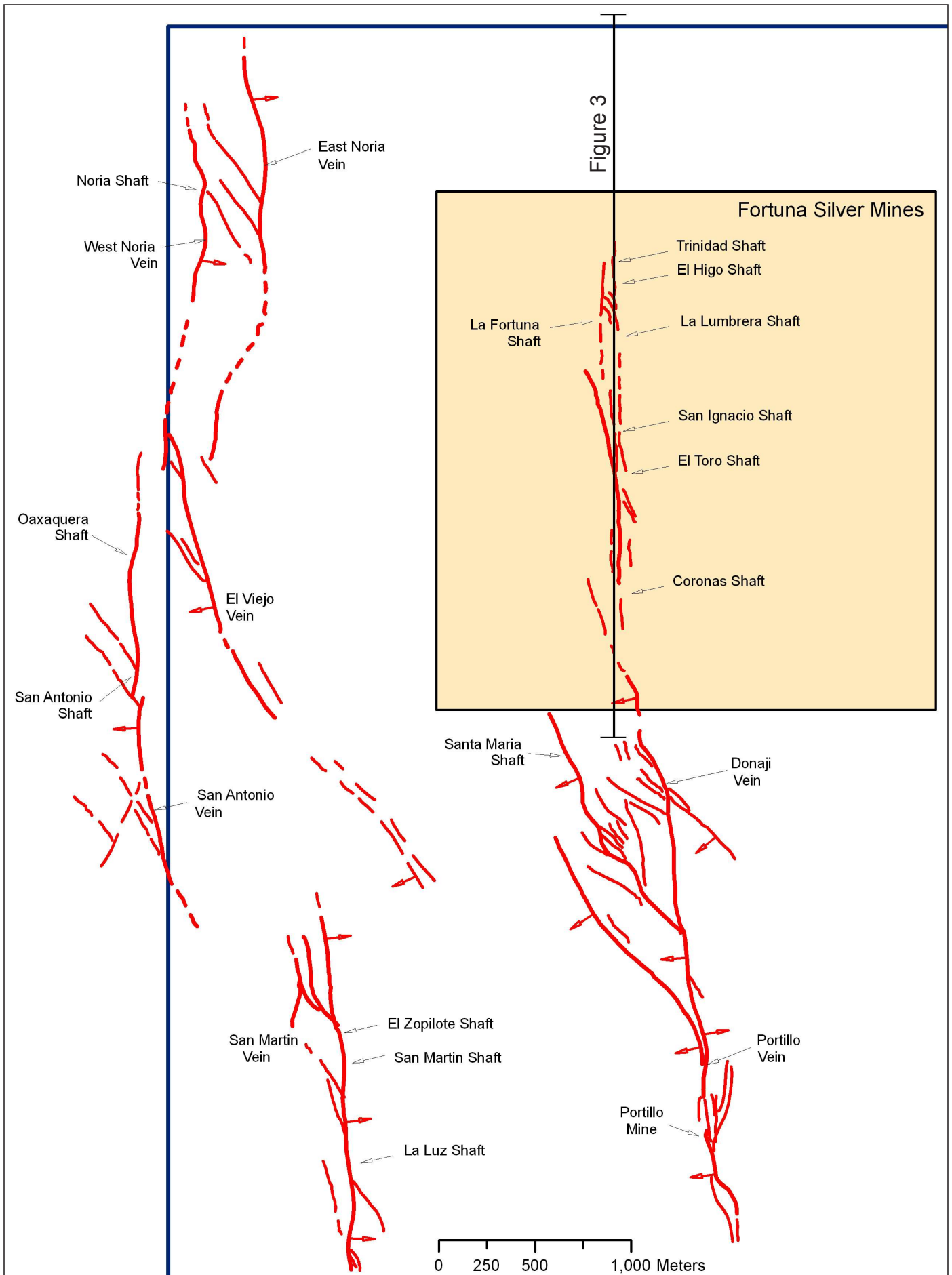
Figure 2 - La Noria and West Taviche Vein Structures
