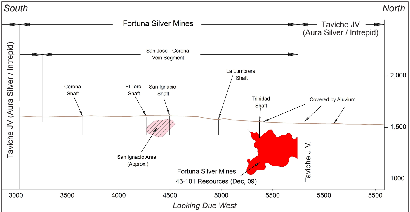
Figure 3 - Longitudinal Section, San Jose
