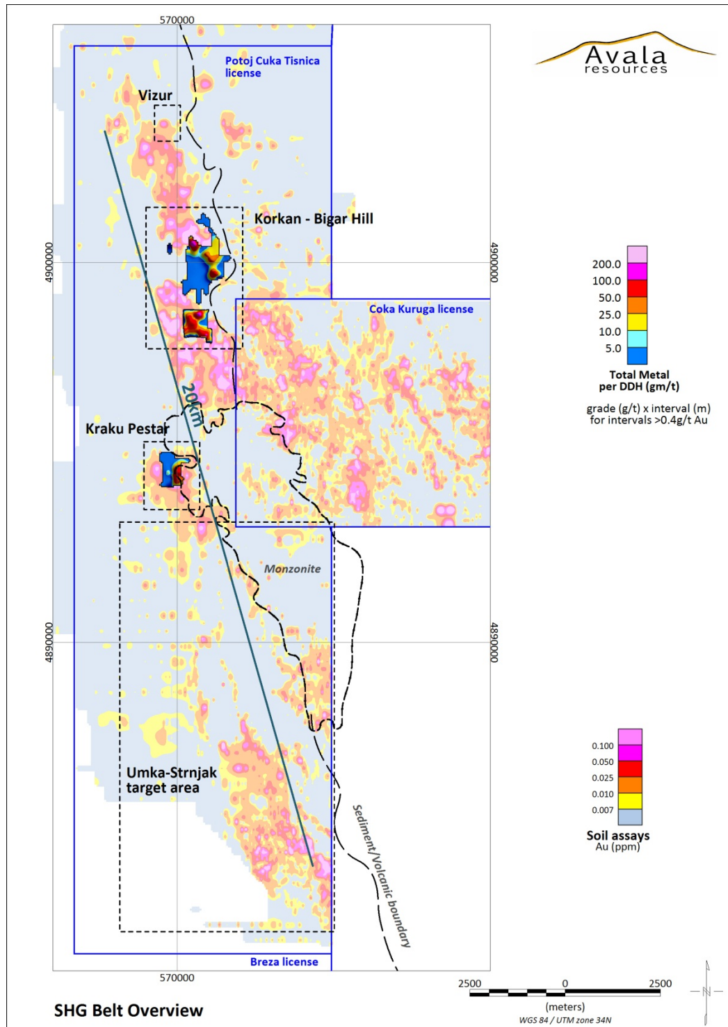
Figure 1: Location of the Korkan-Bigar trend and the Kraku Pestar target area within the 20 kilometer long sediment-hosted gold belt (defined in this image by anomalous gold soil geochemistry). The total metal contour plots for Korkan, Bigar Hill and Kraku Pestar have been superimposed on the sediment-hosted gold belt as defined to date. The Vizur target area has also been highlighted approximately 3 kilometers north of Korkan discovery hole (KODD001).
