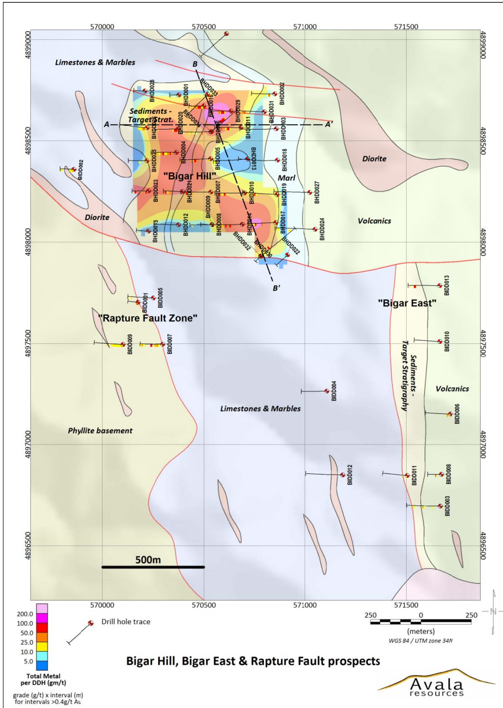
Figure 2: Gram-meter (intervals >0.4g/t Au x thickness), total metal contour plot of all Bigar Hill drilling to date superimposed on a revised target area geology map. The locations of the Rapture Fault Zone and Bigar East have also been highlighted. The section lines A-A' and B-B' relate to Figure 3.
