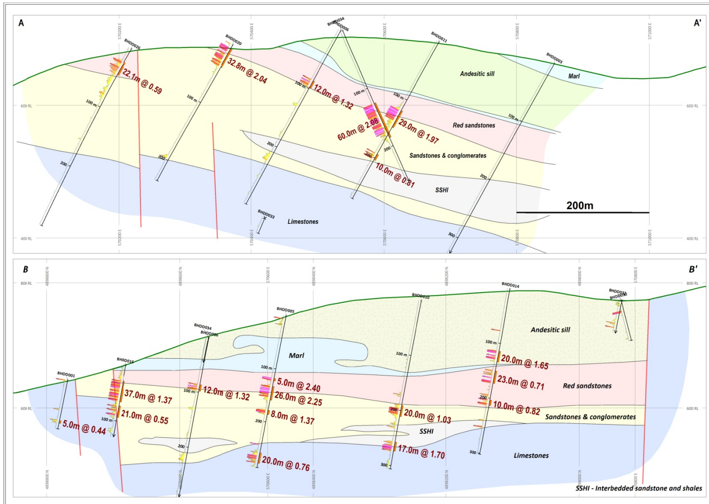
Figure 3: Oblique cross-sections through the Bigar Hill area showing detailed stratigraphy and gold mineralized drill intersections to date (0.4g/t Au cut off). The A-A' section is looking north and the B-B' section is looking approximately east-northeast.
