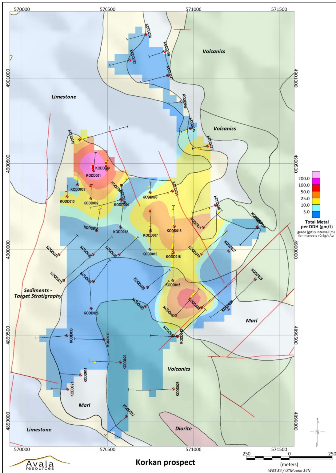
Figure 4: Gram-meter (intervals >0.4g/t Au x thickness), total metal contour plot of all Korkan drilling to date superimposed on a revised target area geology map.
