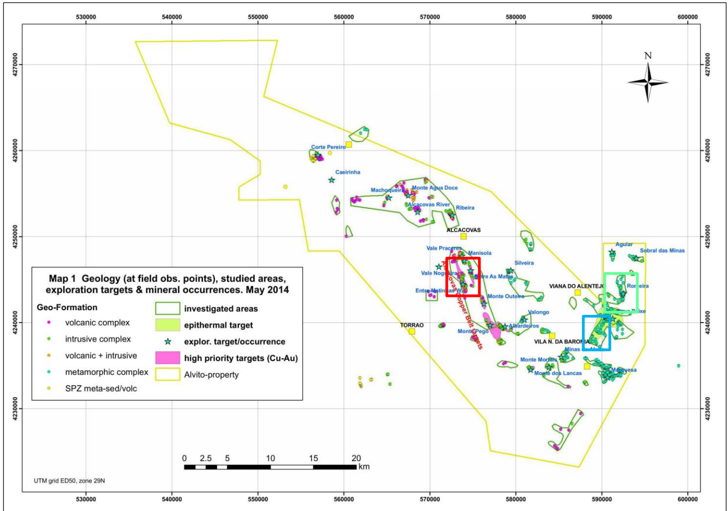
Figure 3. Target areas on Alvito license. Red = Alcaçovas IOCG; Blue = Agua de Peixe epithermal gold-silver target; Green = Agua de Peixe and Romeira silver-lead-zinc massive sulfide targets. New short hole drill sampling planned in Agua de Peixe and Romeira areas.
