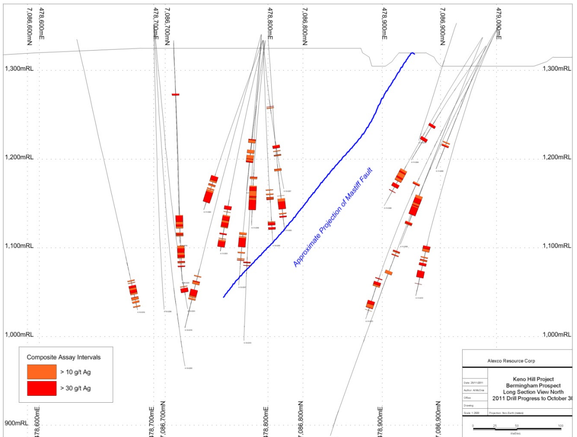
Figure 2 Longitudinal Section 2011 Drill Holes at Birmingham Property Completed to October Showing Greater Than 10 g/t and Greater Than 30 g/t Ag Composite Assay Intervals (viewed to the north).
