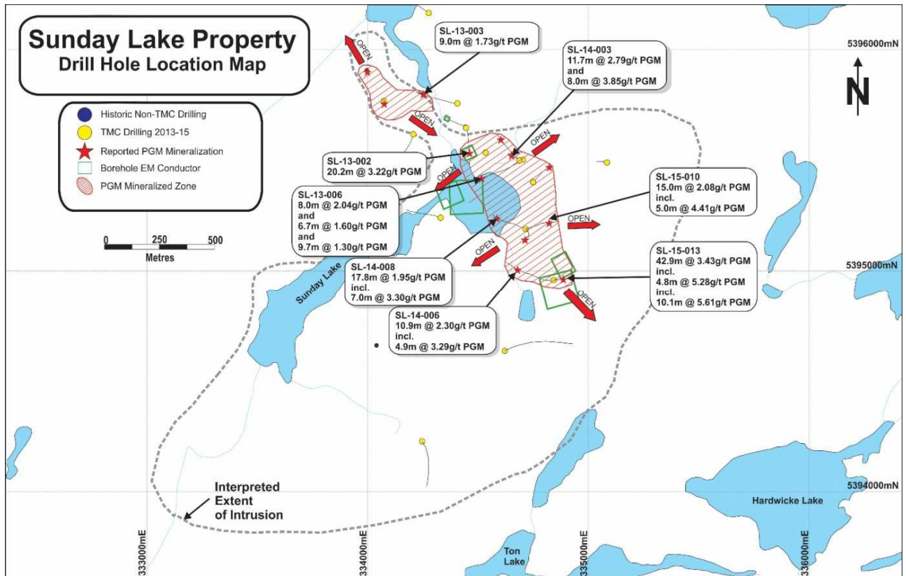
Figure 2. Plan view map showing the location of recent exploration drill holes and the currently known limits to the Sunday Lake PGE-Cu-Ni deposit. Figure modified from the image included in the Transition Metals Corp. news release dated November 16, 2015.
