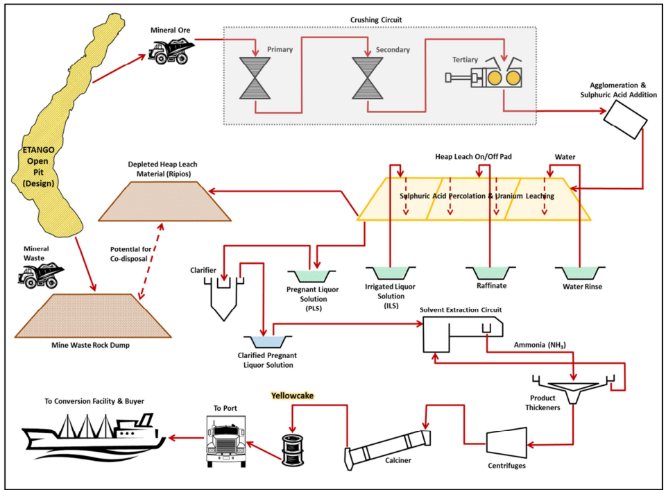
Etango Project - Process Flow Sheet
