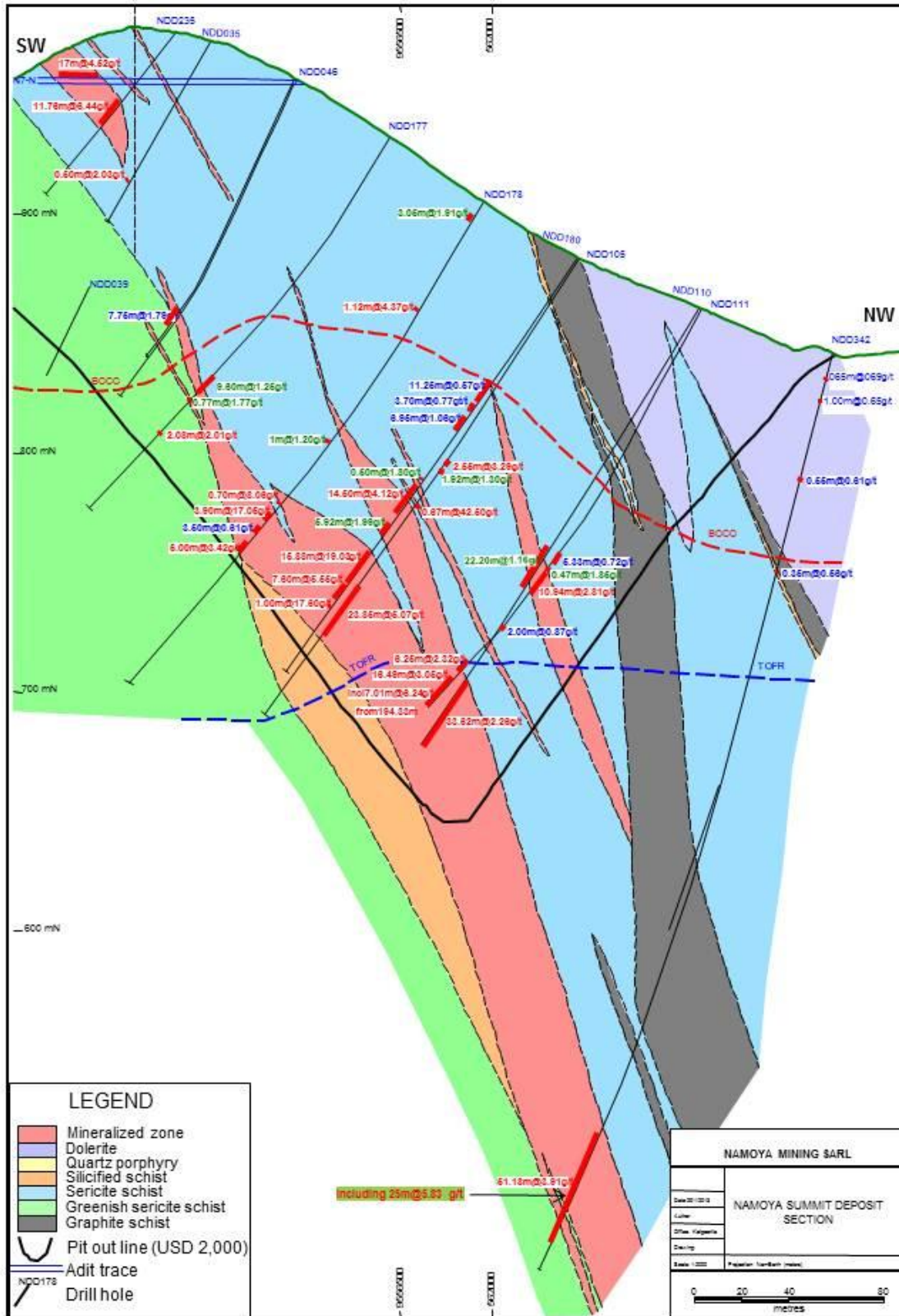
Figure 1 – Namoya cross section
