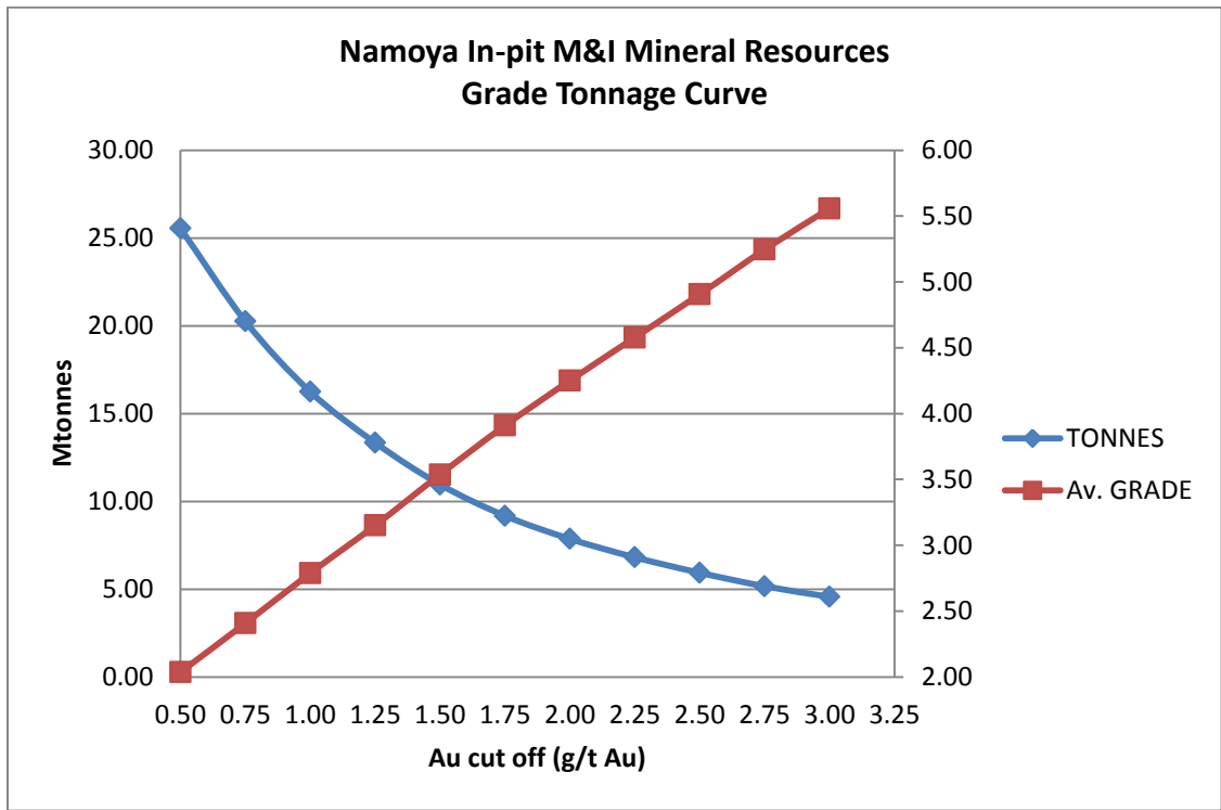
FIGURE 2: Grade Tonnage Curve for the Namoya Project
