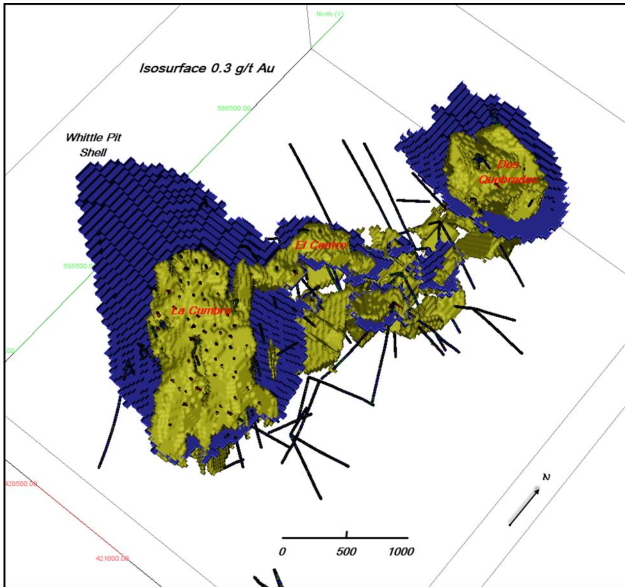
Figure 1 - 3D View Looking Northwest – Blocks Above 0.3 g/t Gold
