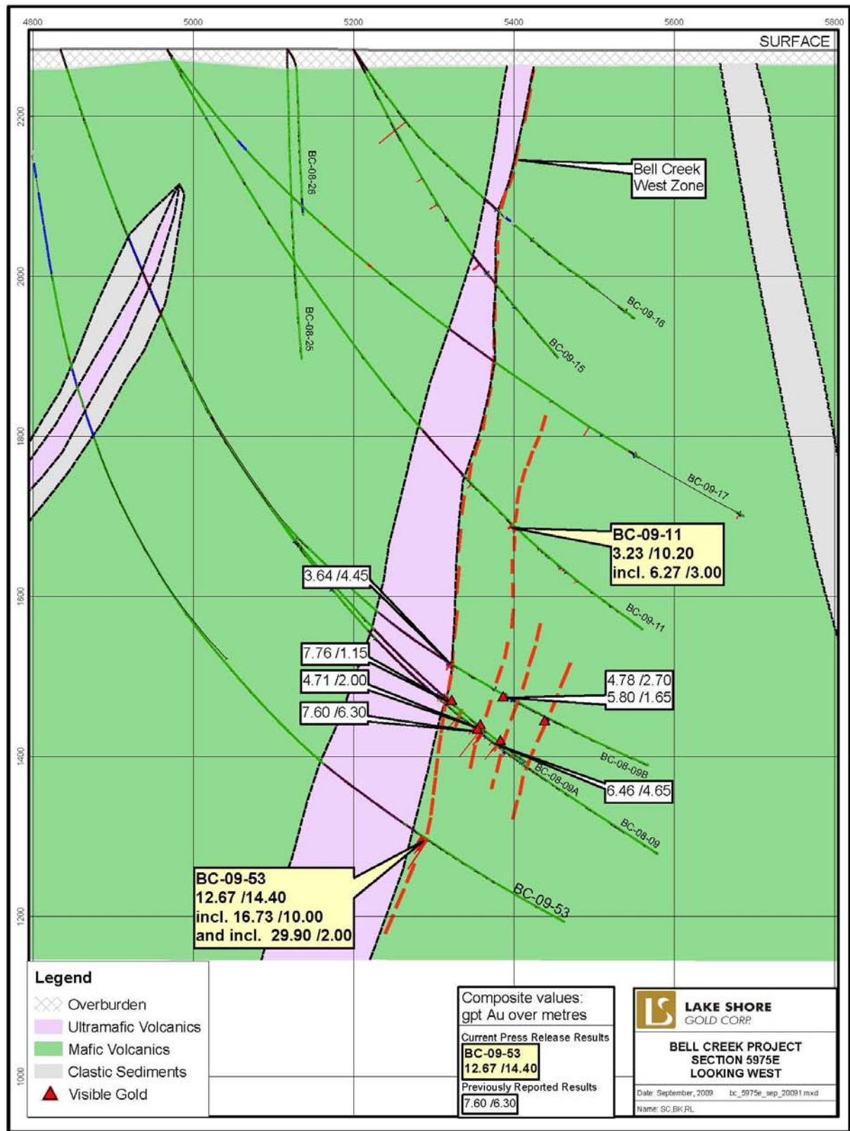
Figure 3. Cross Section
