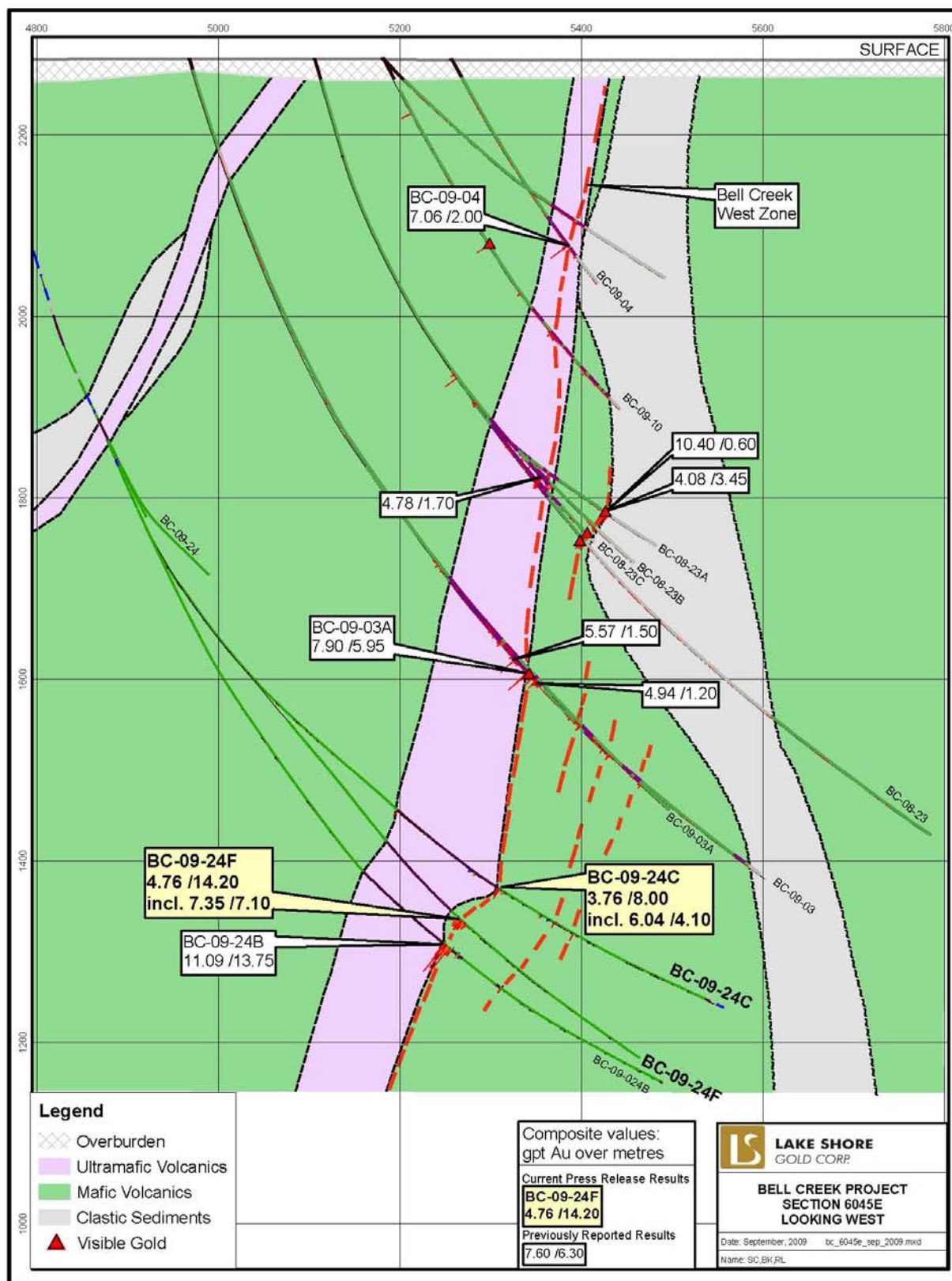
Figure 4. Cross Section (2)
