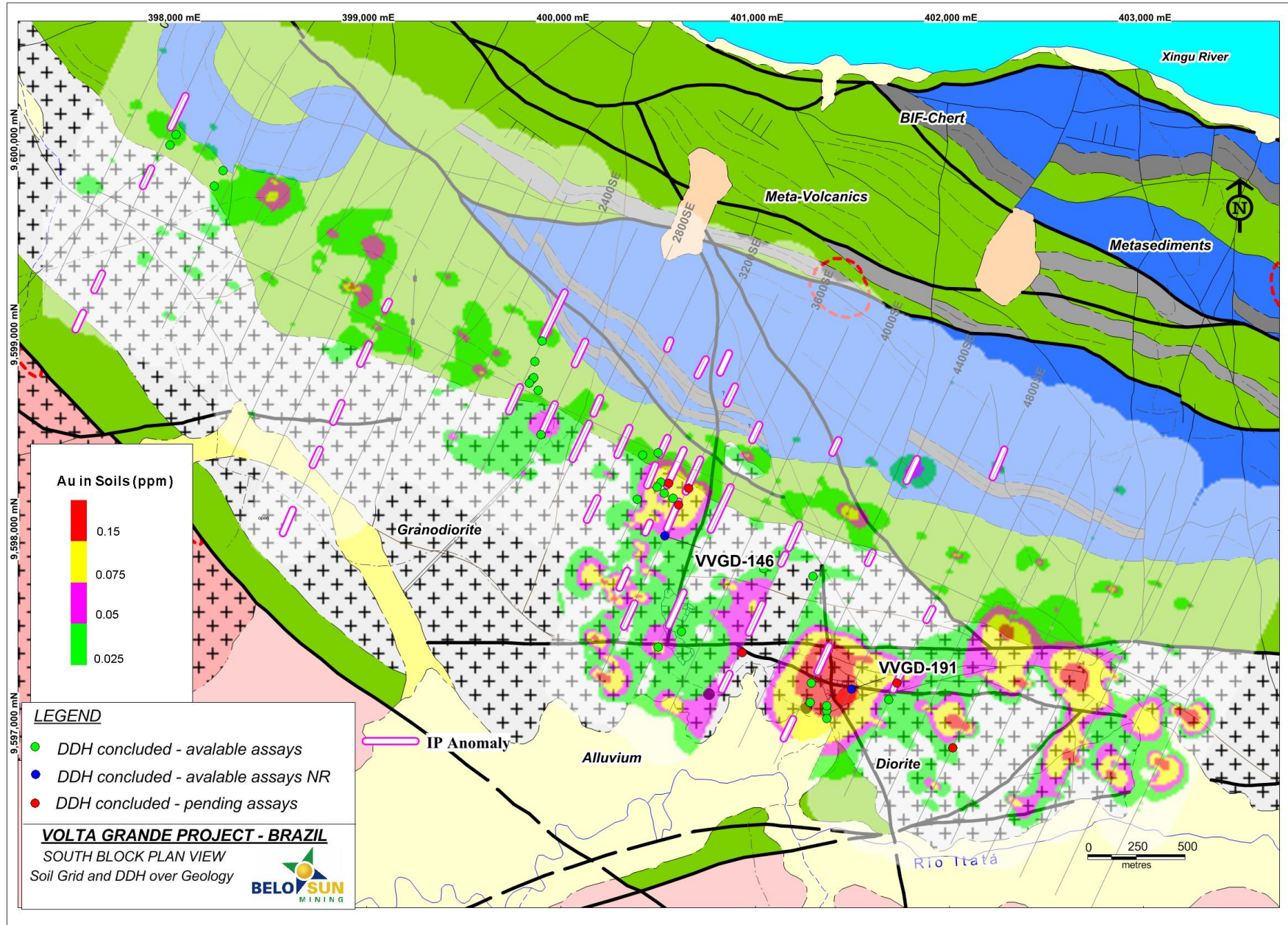
Figure 2 – Volta Grande (South Block) Geological Map
