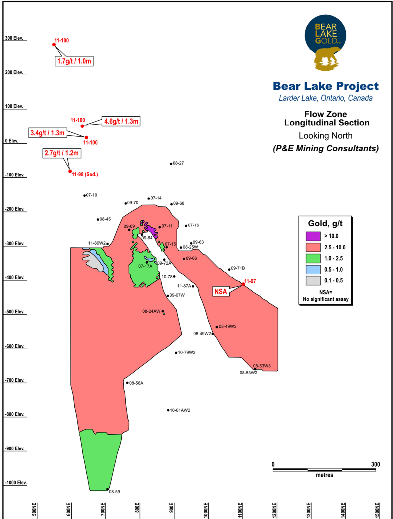
FIGURE 2: BEAR LAKE PROJECT FLOW ZONE LONGITUDINAL SECTION
