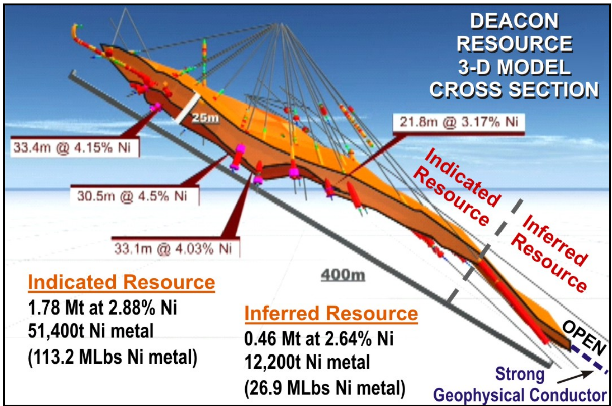
Figure 2: Deacon Resource 3-D Model in Cross Section
