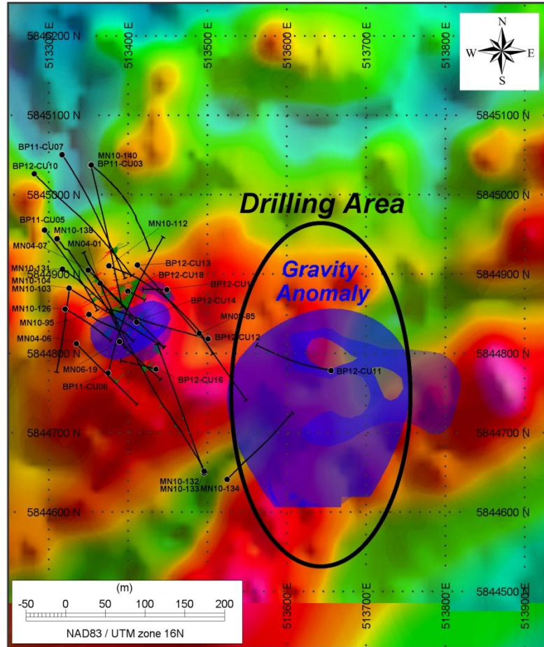
Figure 1: Outline of gravity anomaly and vertical projection of drilling in the Butler 3 area.
