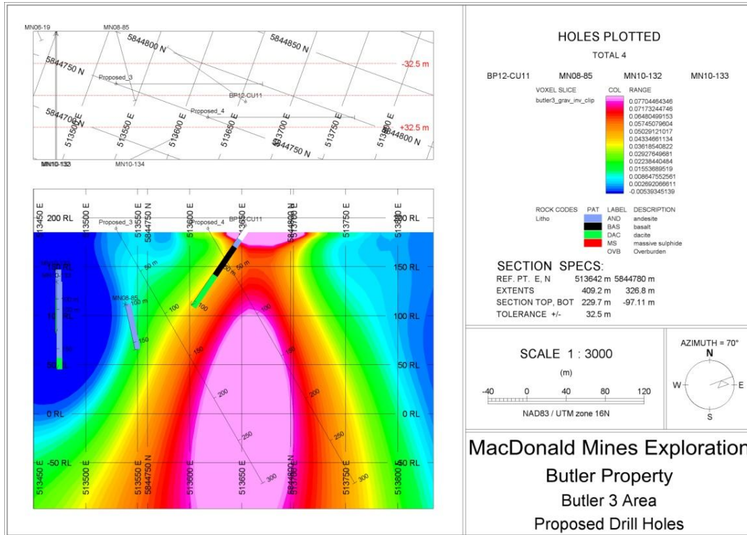
Figure 2: Cross section of gravity anomaly, illustrating proposed holes and BP12 CU11
