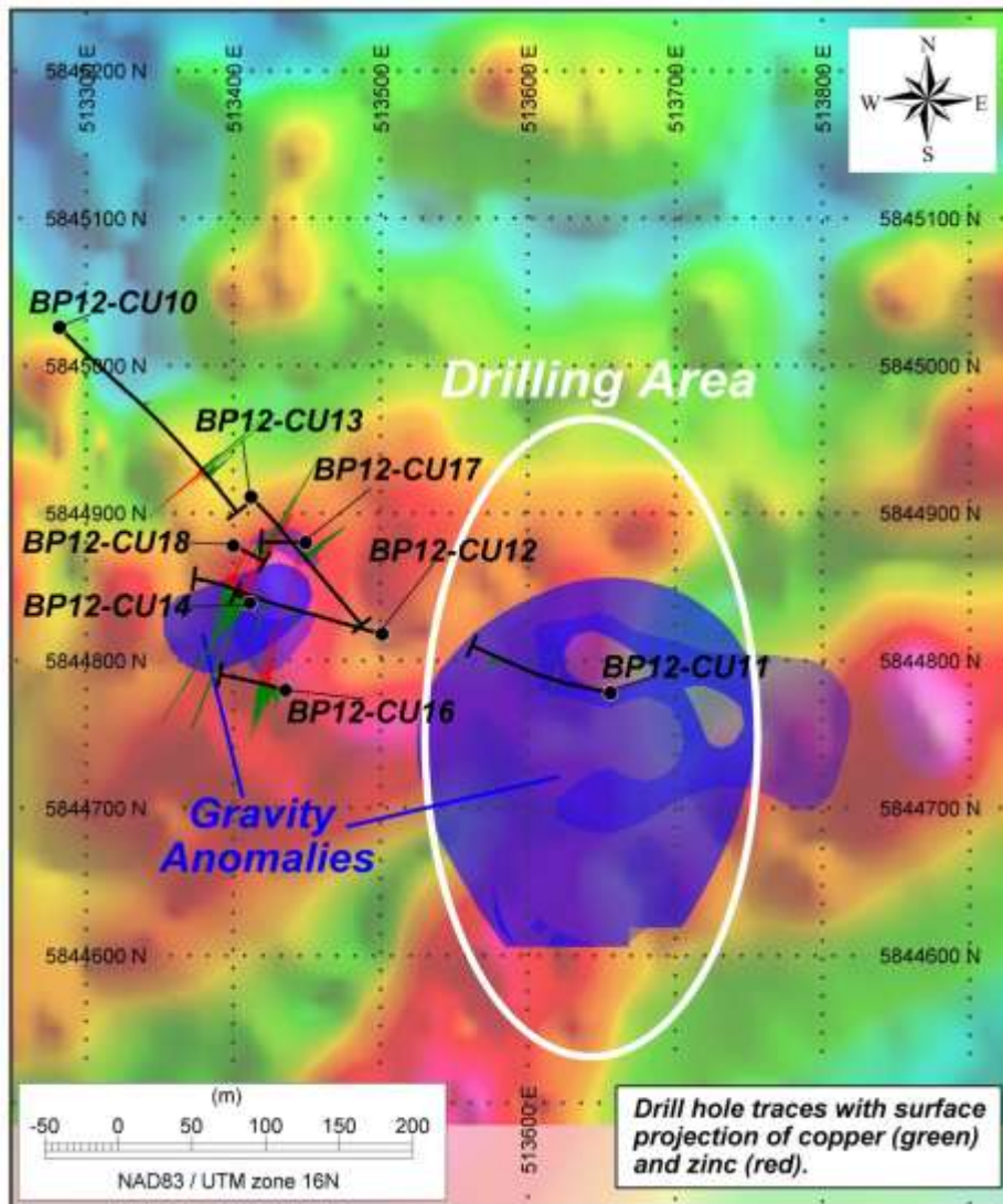
Figure 1: Outline of gravity anomaly and vertical projection of drilling in the Butler 3 area.
