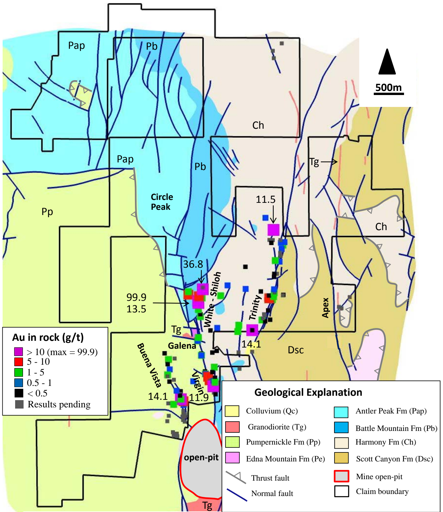
Figure 2: Gold in rock results and geology for the Lewis property of Battle Mountain Gold Inc. Assay values > 10 g/t Au are indicated.
