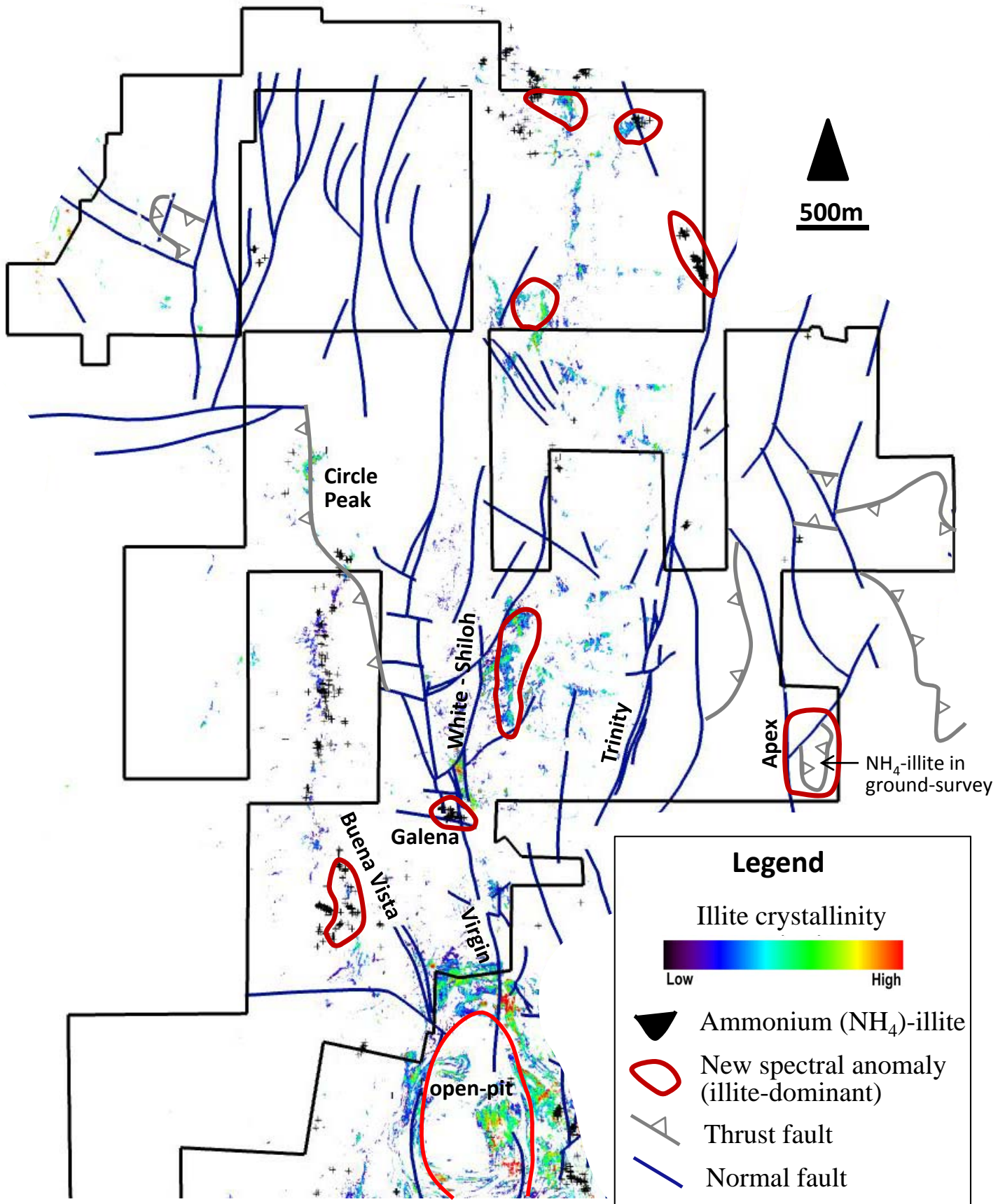
Figure 3: Hyperspectral illite and structural geology of the Lewis property, showing illite crystallinity, ammonium-illite and new spectral anomalies.
