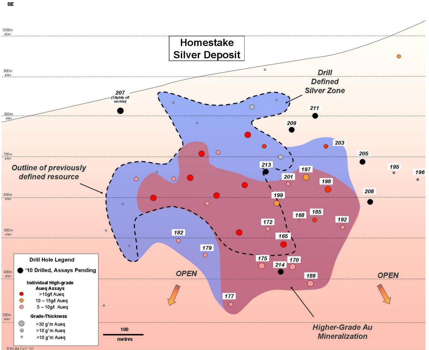
Figure 1: Representative Longitudinal Section of the Homestake Silver Deposit
