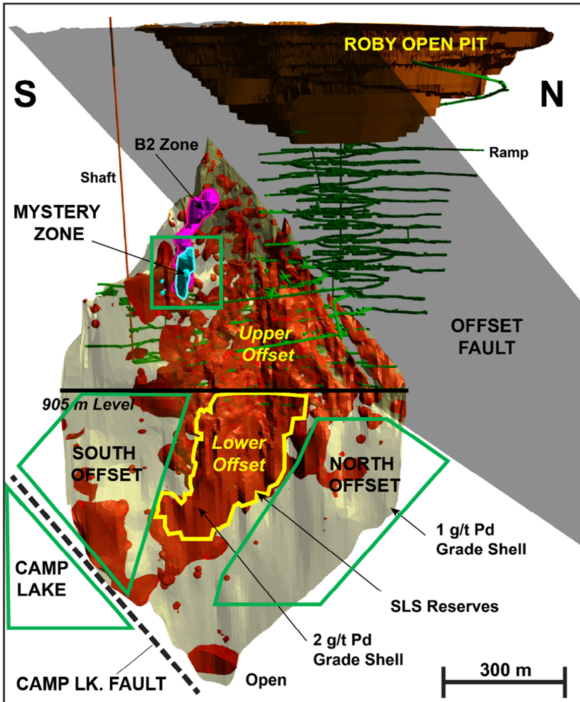
Figure 3. Oblique longitudinal projection, looking west, and showing the current priority underground resource extension and exploration targets on the Lac des Iles mine property, including: Mystery Zone; South Offset; North Offset; and, Camp Lake.
