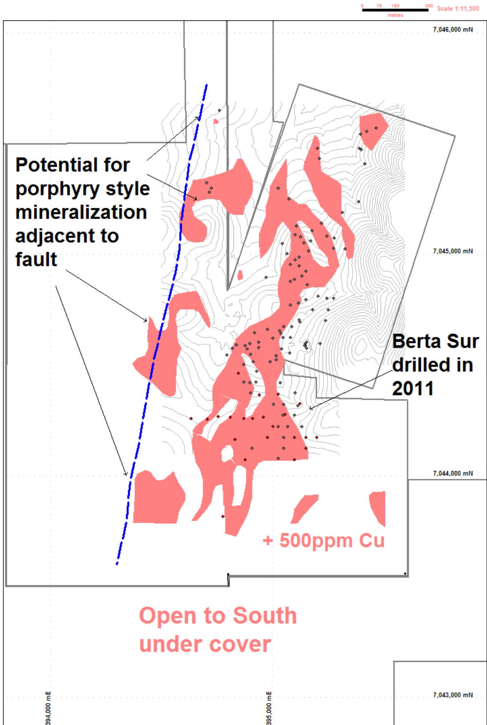
Figure 1. Berta Copper Geochemistry
