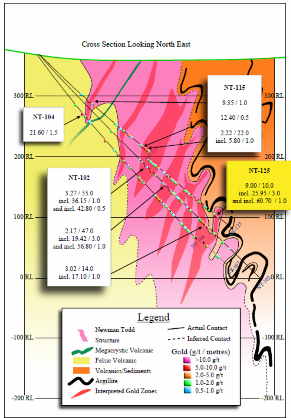
Figure 2: Newman Todd Cross-Section Looking North-East
