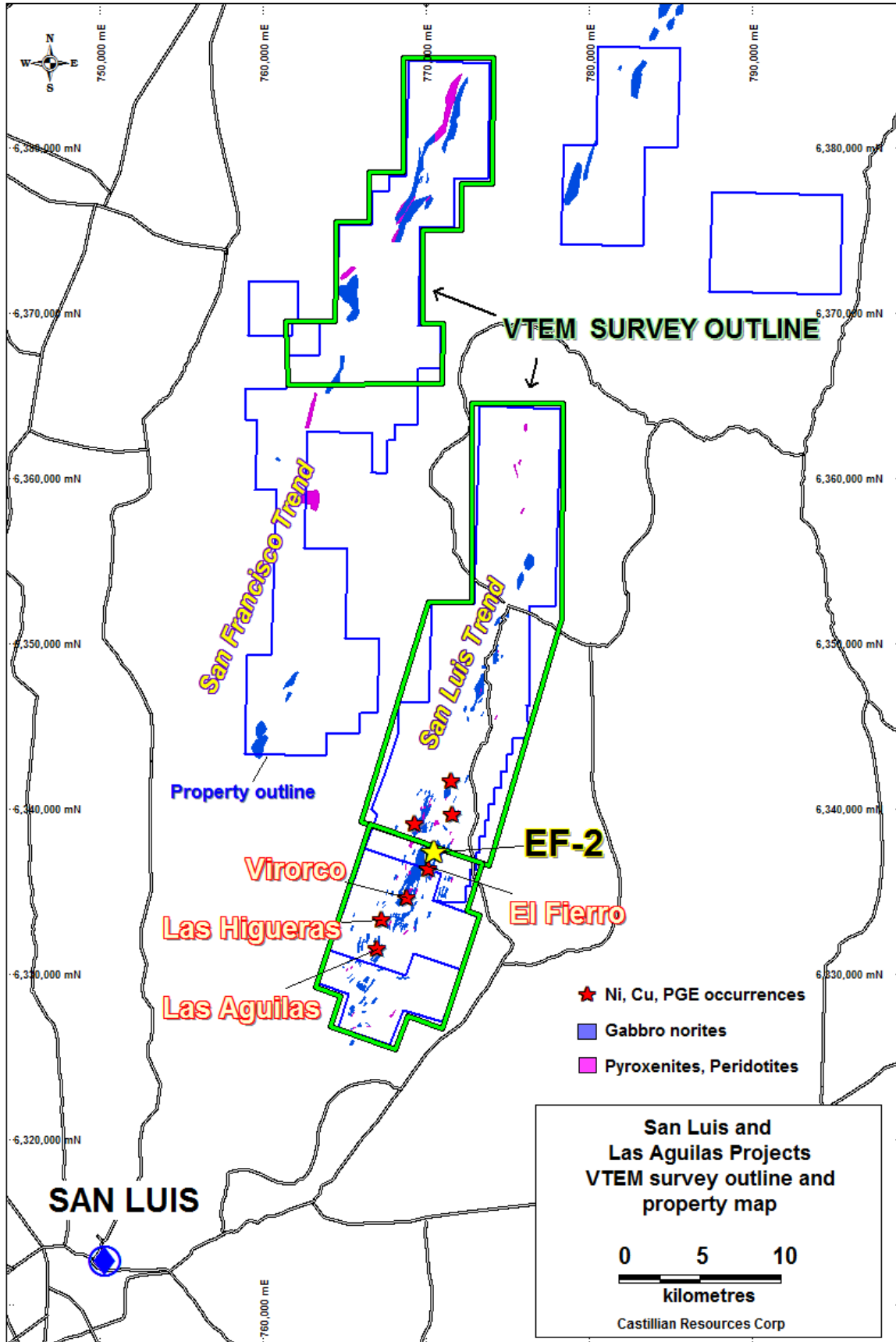
Figure 3: Map showing the outline of the VTEM Airborne Survey and location of the EF-2 Gossan relative to the Las Aguilas Deposits and other known nickel-copper-PGE occurrences in the project area.
