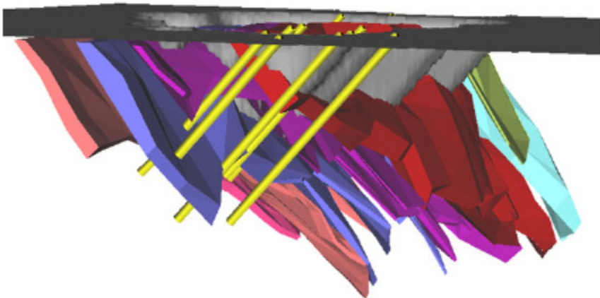
K1-1 3D model of pits and mineralization with holes K-11-33 thru K-11-42
