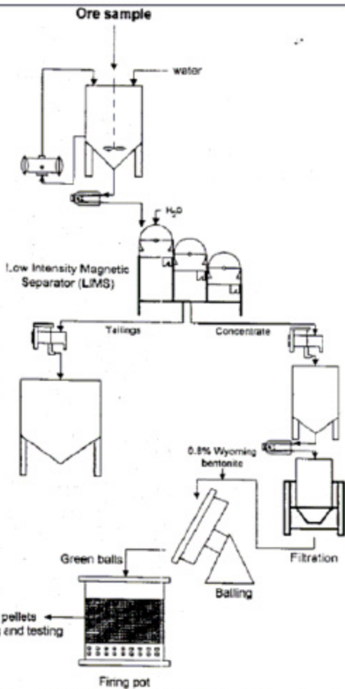
Fig.1: Beneficiation and Pelletizing Flowsheet (after Met-Chem)
