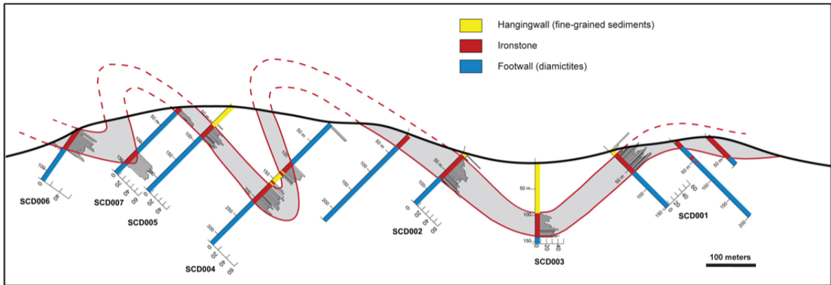
FIGURE 2: Cross-section 1007170N looking north for holes SCD-001 to SCD-007. Analytical results for iron are represented as bars on right side of drillhole traces. West-directed thrust faulting has resulted in a moderate folded geometry. Fault traces and minor displacements have been omitted for clarity (thickening and thinning of the ironstone is most likely related to faulting). Ironstones sub-cropping on dip-slopes (central and eastern zones) provide excellent potential for zero-strip extraction zones.
