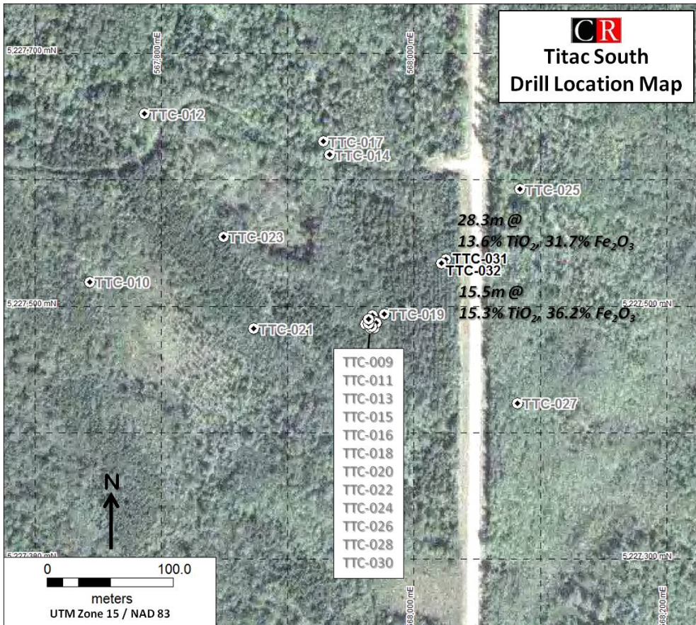
Figure 2: Drillhole locations at the TiTac Ferro-Titanium deposit
