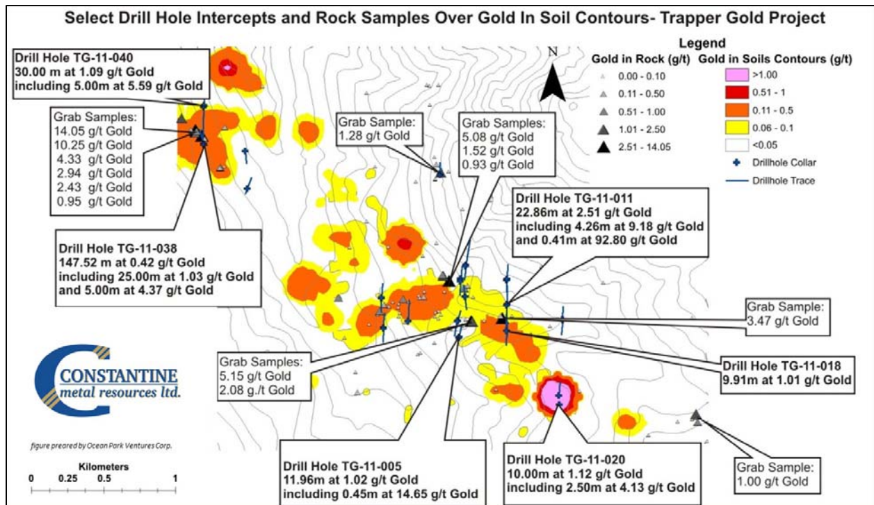
Figure 1. Map of Main Gold zone with highlight results of 2011 exploration program.
