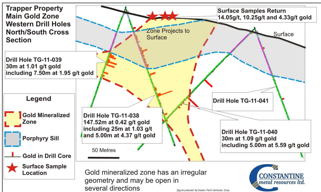
Figure 2. North-south cross section of the Main Gold zone (west) showing gold intercepts in drill core.
