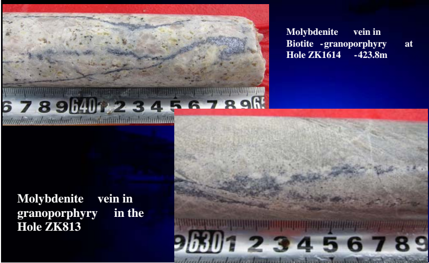
Photo 1, Molybdenite vein in granoporphyry from the core of Hole ZK813 and Hole ZK1614 at Jiama Project
